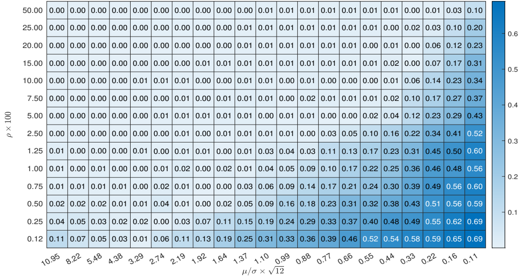
Figure 6: Comparison between \hat{S}^* and S^*
